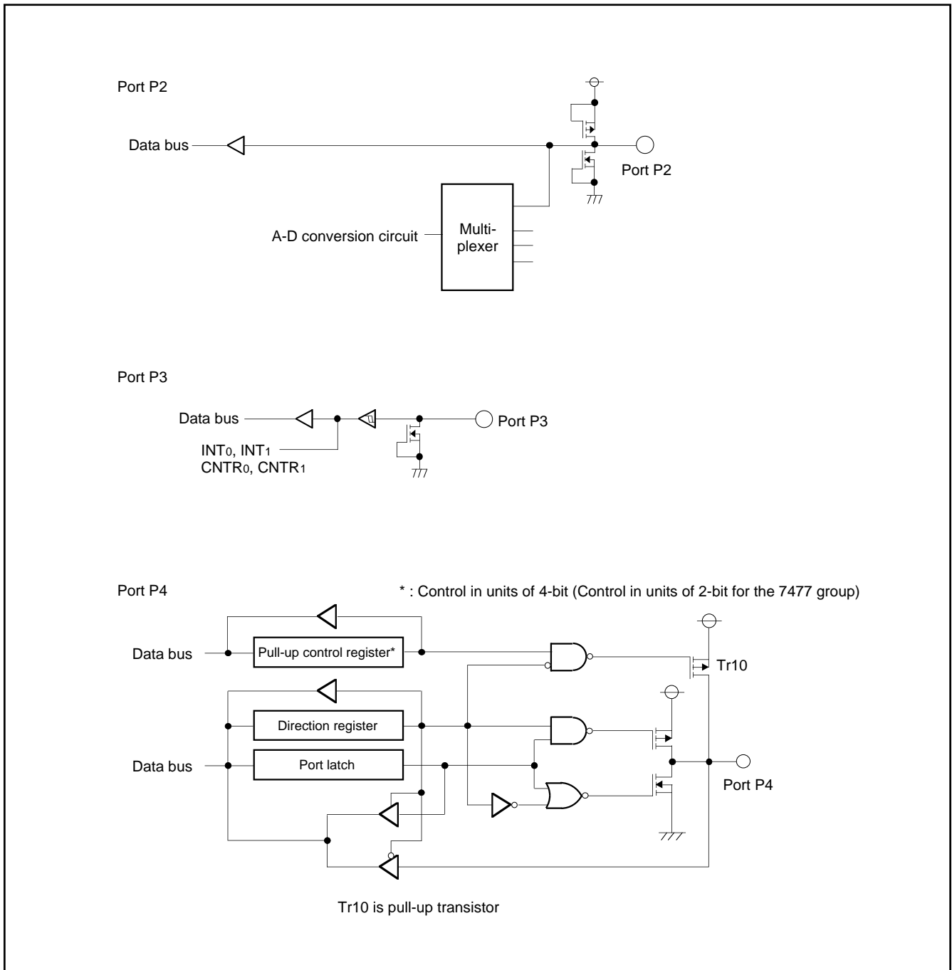
Fig. 21 Block diagram of ports P2 – P4
