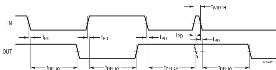
Figure 5. Both Edges Delayed Timing Diagram (LTC6994-2, POL = 0 )
