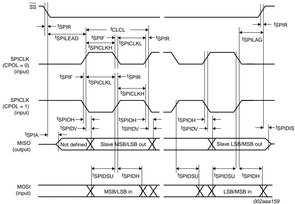
Fig 33. SPI slave timing (CPHA = '1')
