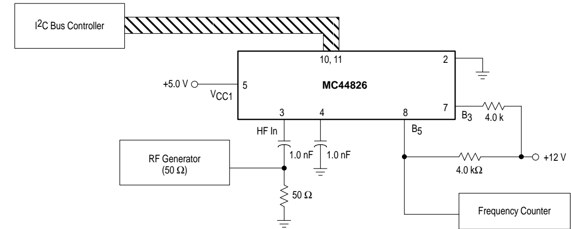
Figure 2. RF Sensitivity Test Circuit
