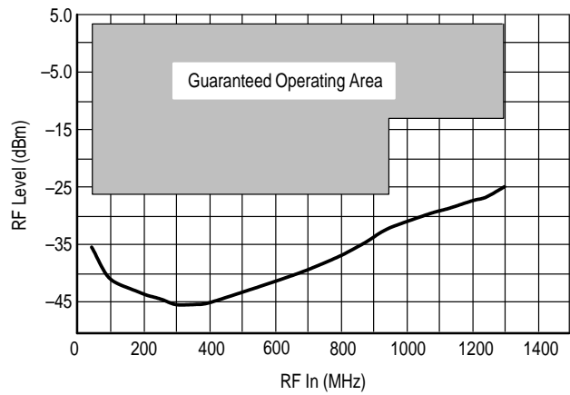
Figure 1. Typical Prescaler Input Sensitivity
