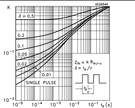
Figure 5. Thermal impedance for TO-220FP
