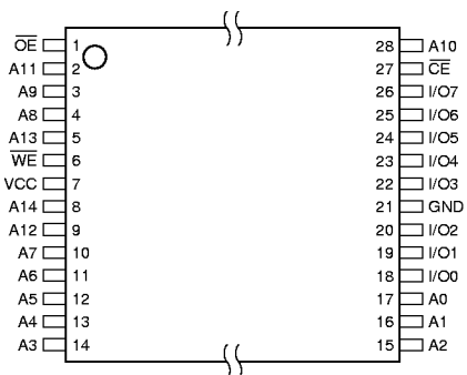
LCC, PLCC Top View
