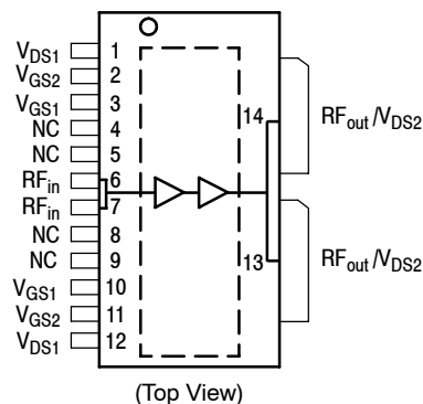
Figure 2. Pin Connections
