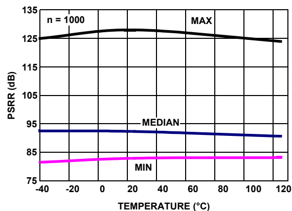
FIGURE 42. PSRR vs TEMPERATURE, V_+ , V_- = \pm 1.2V TO \pm 2.5V
