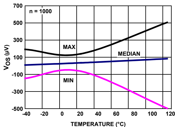
FIGURE 38. ISL28270, ISL28470 V_{OS} vs TEMPERATURE, V_+ , V_- = \pm 1.2V
