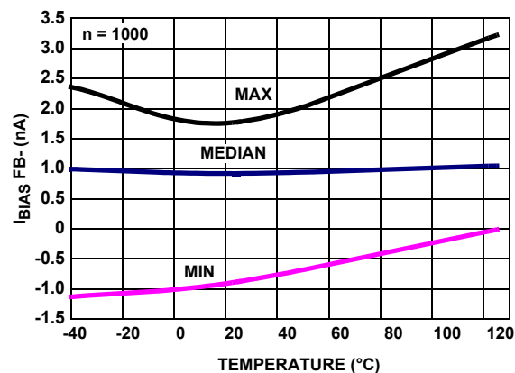
FIGURE 32. I_{BIAS\ FB-} vs TEMPERATURE, V_+ , V_- = \pm 1.2V
