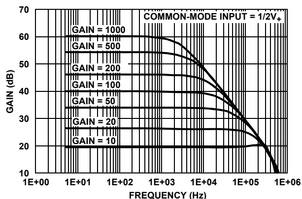
FIGURE 4. ISL28273 FREQUENCY RESPONSE vs CLOSED LOOP GAIN, V_+ = 5V , V_{CM} = 1/2V_+
