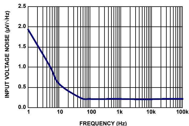
FIGURE 16. ISL28273 INPUT VOLTAGE NOISE SPECTRAL DENSITY (GAIN = 10)
