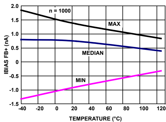
FIGURE 26. I_{BIAS\ FB+} vs TEMPERATURE, V_+ , V_- = \pm 2.5V
