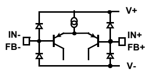
CIRCUIT 1B
