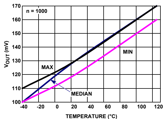
FIGURE 46. V_{OUT} LOW vs TEMPERATURE, R_L = 1k , V_+ , V_- = \pm 2.5V
