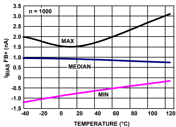
FIGURE 30. I_{BIAS\ FB+} vs TEMPERATURE, V_+ , V_- = \pm 1.2V
