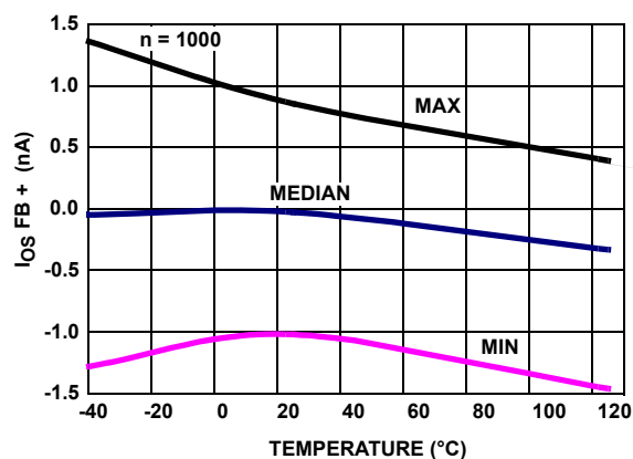
FIGURE 36. I_{OS} FB+ vs TEMPERATURE, V_+ , V_- = \pm 1.2V
