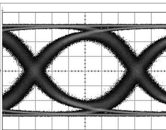
Figure 9-4. TL = 35-Inch 4-Mil FR4 Trace
