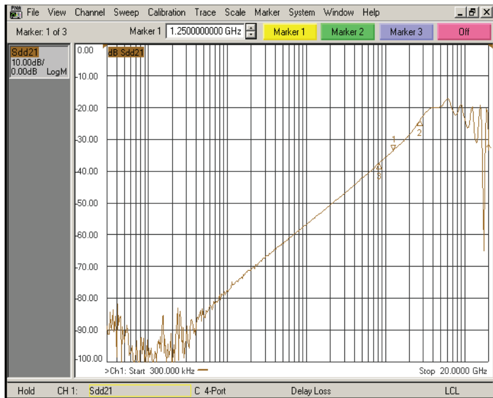
Fig 5. Off Isolation
