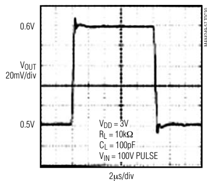
MAX4250-MAX4254 SMALL-SIGNAL PULSE RESPONSE
