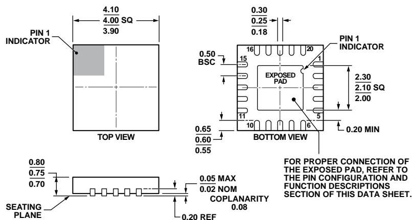
Figure 15. 20-Lead Lead Frame Chip Scale Package [LFCSP_WQ] 4 mm × 4 mm Body, Very Very Thin Quad (CP-20-6) Dimensions shown in millimeters
