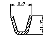
SECT "A"-"A"
