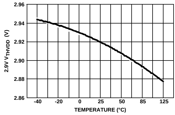
FIGURE 8. ISL8800x 2.9V V_{THVDD} vs TEMPERATURE
