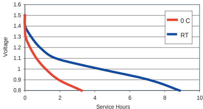
TYPICAL FLASHLIGHT TEST AT 21°C AND 0°C
