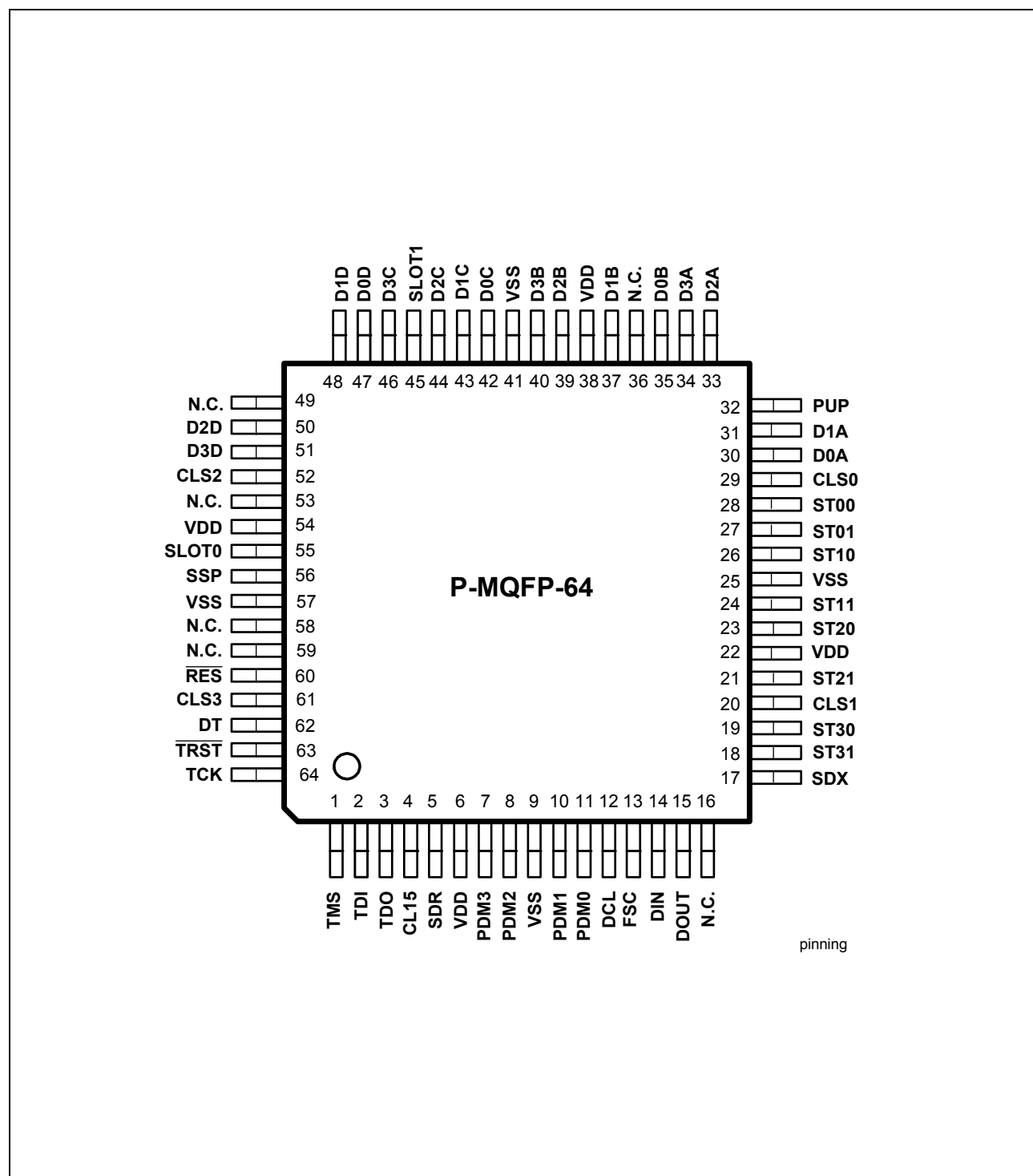
Figure 6 Pin Configuration
