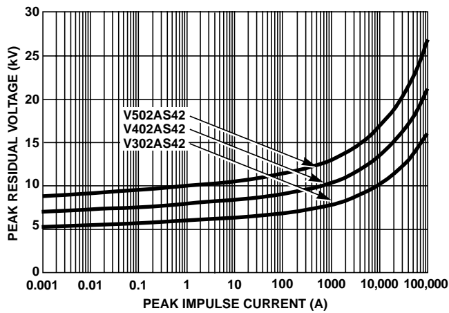
FIGURE 3. V-I CHARACTERISTIC AS42 SIZE
