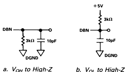
Figure 2. Load Circuits for Data Hold Time Test
