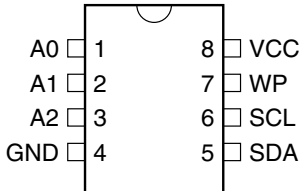
8-pin PDIP
