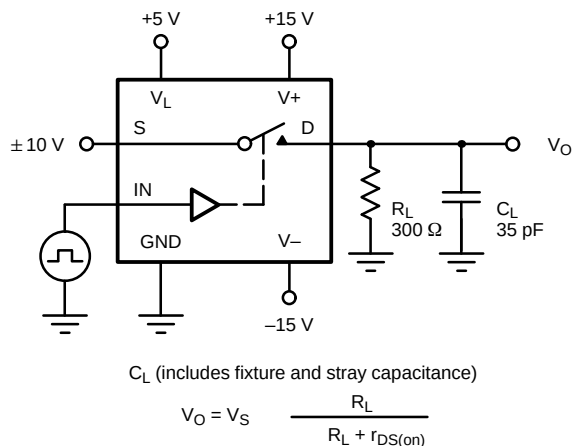
FIGURE 2. Switching Time
