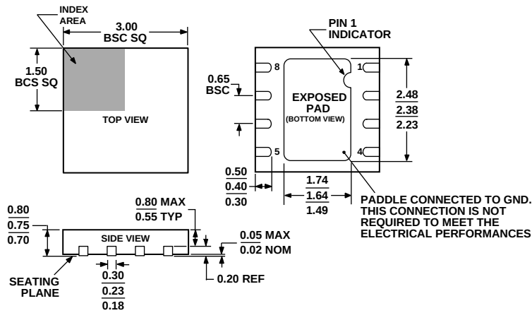
Figure 27. 8-Terminal Quad Flat No Lead Package [QFN (LFCSP)] 3 mm x 3 mm Body (CP-8-9)
