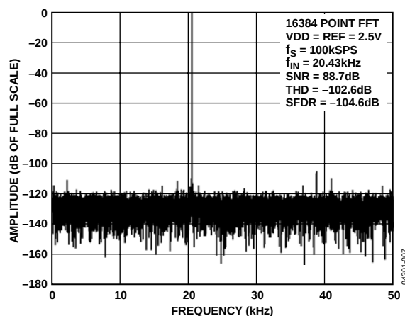
Figure 12. FFT Plot
