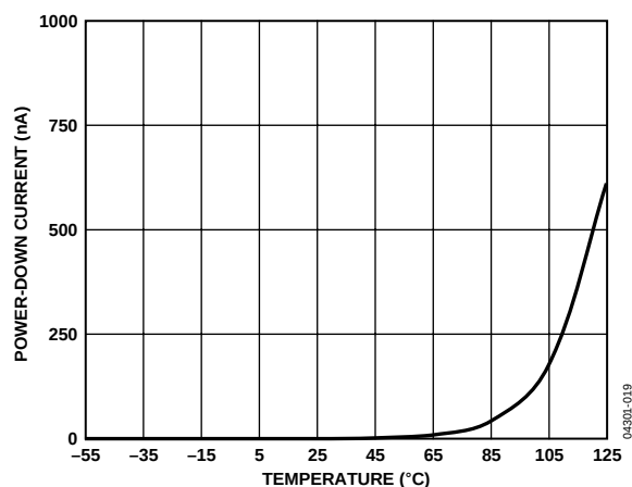
Figure 18. Power-Down Currents vs. Temperature
