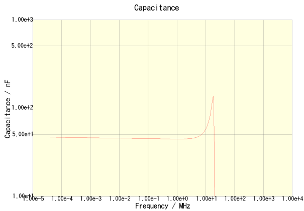
C3225X7R2J473K200AA
