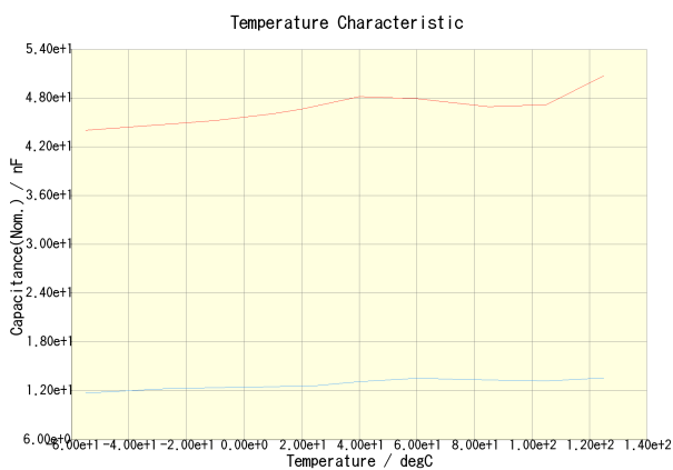
C3225X7R2J473K200AA(DC Bias = 0V) C3225X7R2J473K200AA(DC Bias = 315V)
