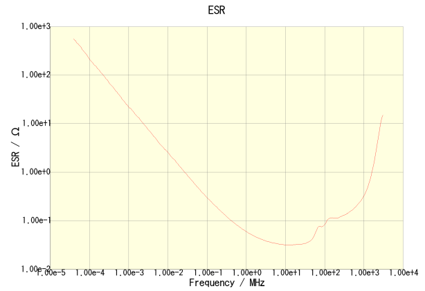
C3225X7R2J473K200AA
