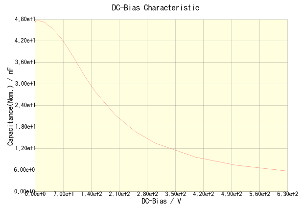
C3225X7R2J473K200AA
