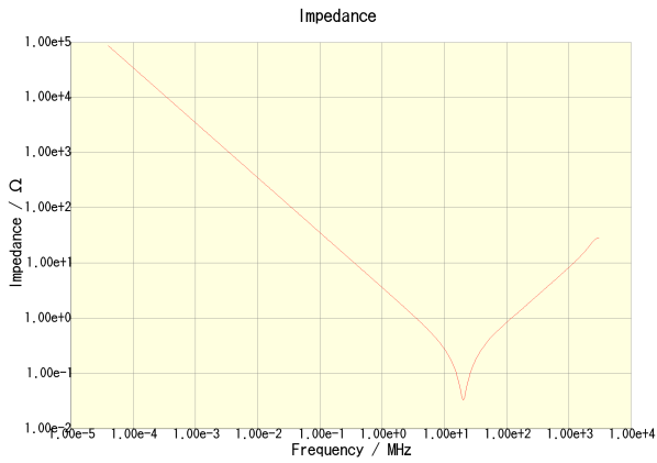
C3225X7R2J473K200AA
