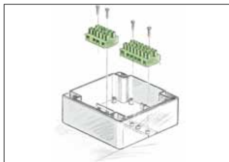
Bosses for terminal blocks (type KL 16, Wieleland).
