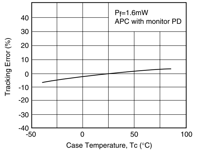
Fig. 6 Tracking Characteristics
