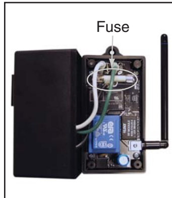
Figure 4: FCTN-WALL-418 Fuse
