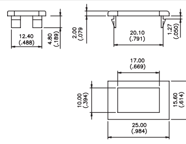
U4602 for SW, SWW & SY models (Black standard - consult factory for others)
