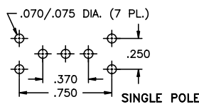
SINGLE POLE
