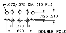
DOUBLE POLE
