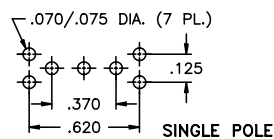
SINGLE POLE
