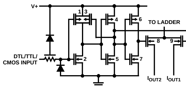
FIGURE 1. CMOS SWITCH
