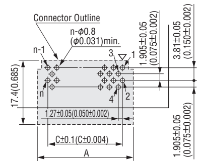
For 26,30,34,50 pins
