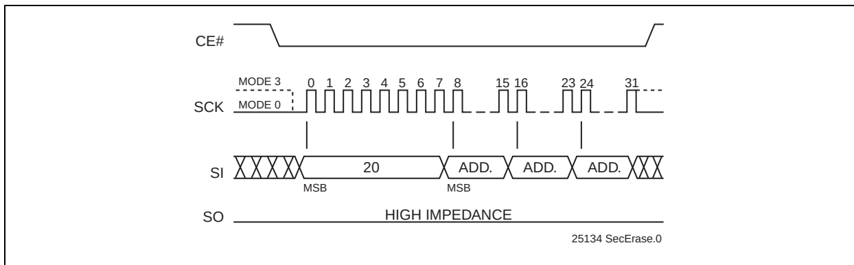
FIGURE 4-10: SECTOR-ERASE SEQUENCE
