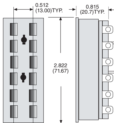
TRF - 12 PIN
