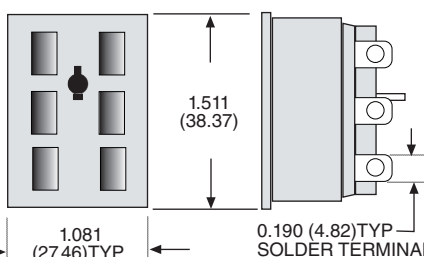
TRF - 6 PIN
