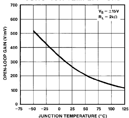
OPEN-LOOP GAIN vs JUNCTION TEMPERATURE
