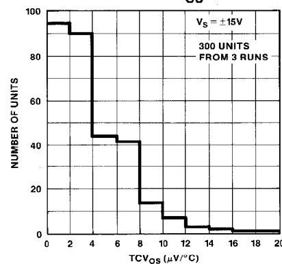
TYPICAL DISTRIBUTION OF TCVOS
