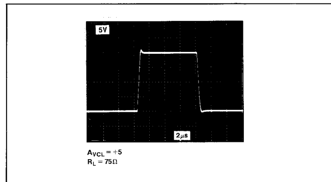
FIGURE 9: Output Buffer Large-Signal Response
