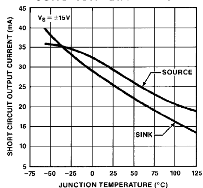
SHORT CIRCUIT OUTPUT CURRENT vs JUNCTION TEMPERATURE
