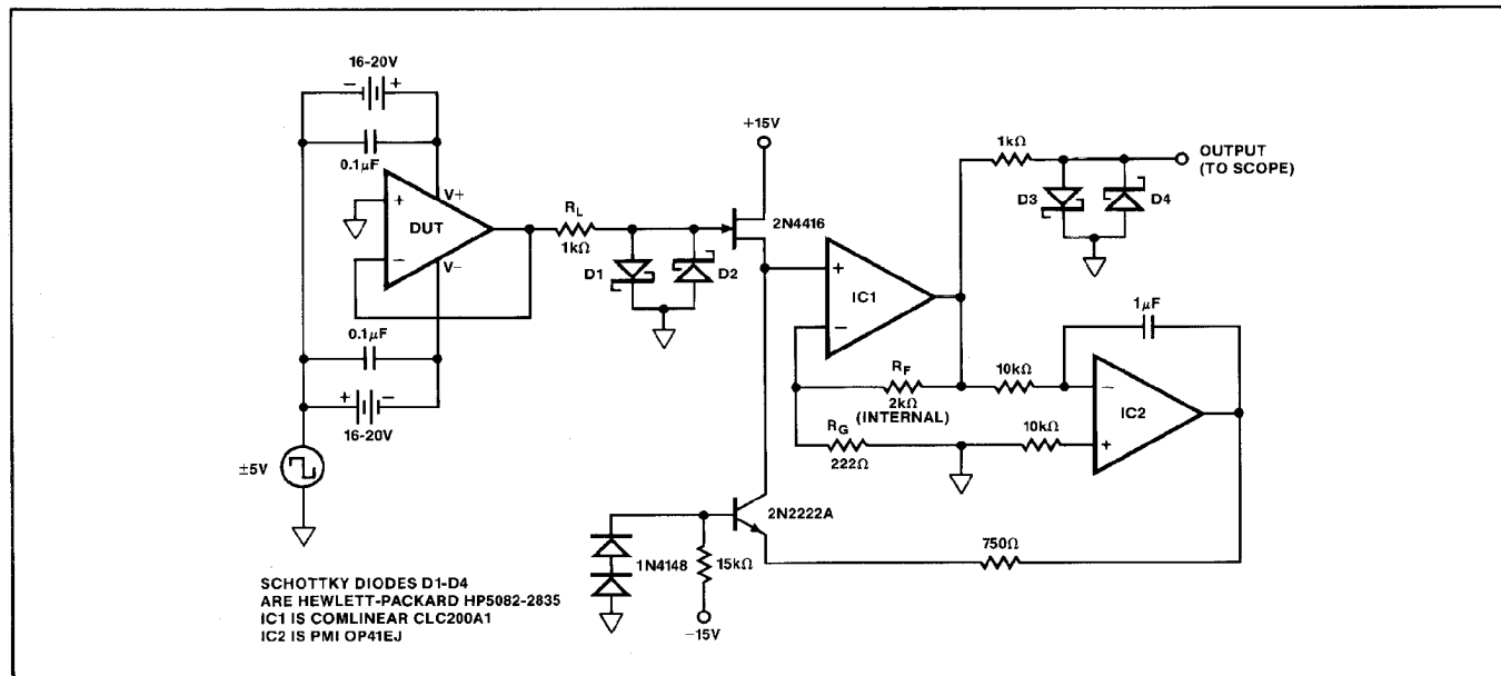
FIGURE 4: Settling-Time Test Fixture
