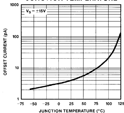
OFFSET CURRENT vs JUNCTION TEMPERATURE
