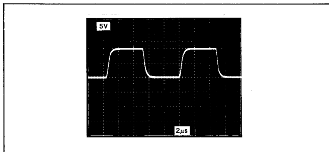
FIGURE 7: DAC Output Amplifier Response (PM-7545 DAC)
