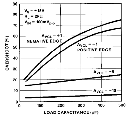
SMALL-SIGNAL OVERSHOOT vs LOAD CAPACITANCE
