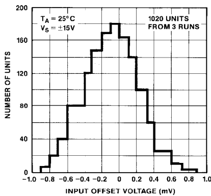
TYPICAL DISTRIBUTION OF INPUT OFFSET VOLTAGE
