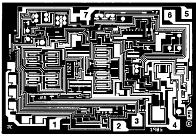
DIE SIZE 0.098 × 0.070 inch, 6860 sq. mils (2.49 × 1.78 mm, 4.43 sq. mm)
