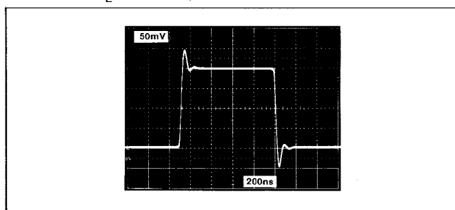
FIGURE 1: Small-Signal Transient Response, Z_L = 2k\Omega || 75pF
