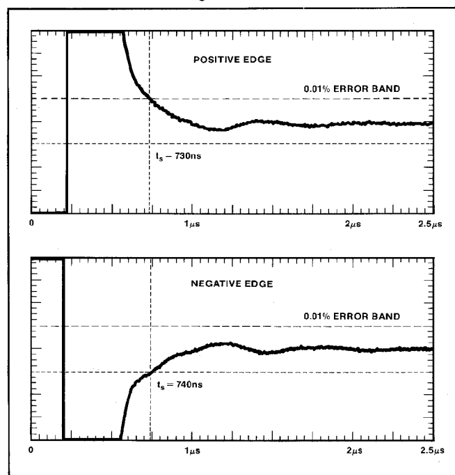
FIGURE 5: OP-42 Settling-Characteristics
