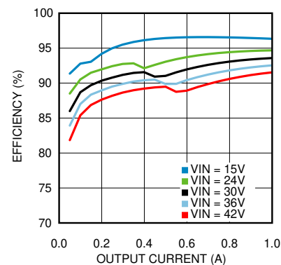
Efficiency V OUT = 12 V, T A = 25°C
