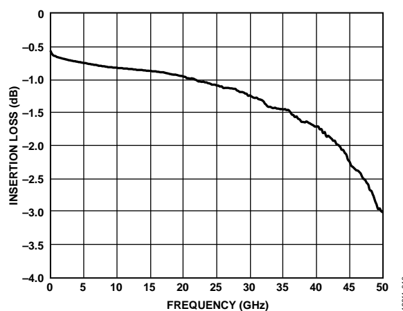
Figure 10. Insertion Loss vs. Frequency Without Impedance Match
