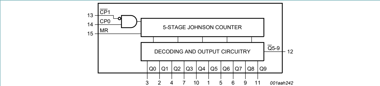
Fig. 1. Functional diagram
