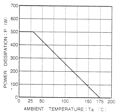
Fig. 4 Derating curve
