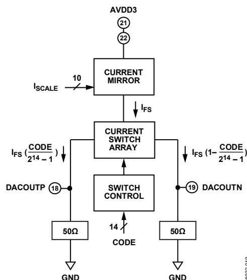
Figure 45. DAC Output Pins
