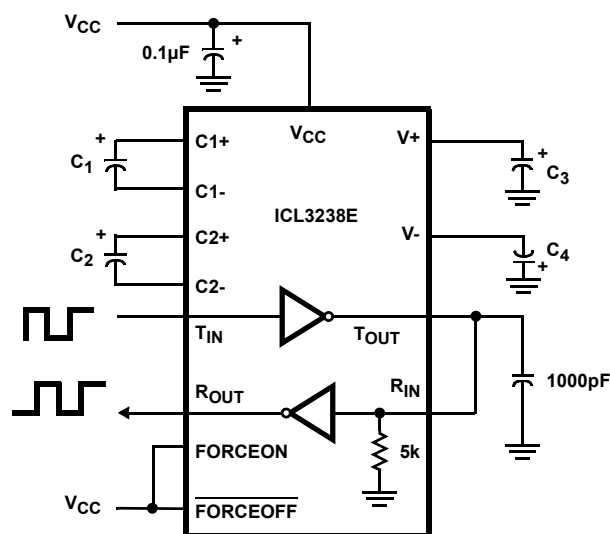
FIGURE 11. TRANSMITTER LOOPBACK TEST CIRCUIT
