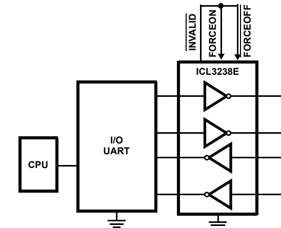
FIGURE 9. CONNECTIONS FOR AUTOMATIC POWERDOWN WHEN NO VALID RECEIVER SIGNALS ARE PRESENT
