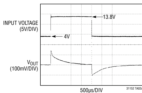
Fast (10µs) Line Transient from V_{IN} = 4V to 13.8V
