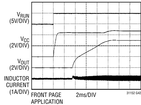
Soft-Start Waveforms
