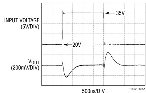
Fast (20 \mu s) Input Voltage Transient, V_{IN} = 20V to 35V
