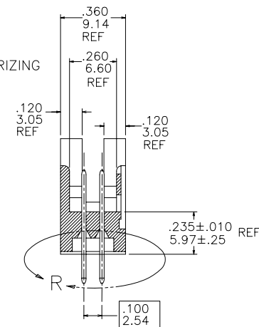
SECTION F-F
