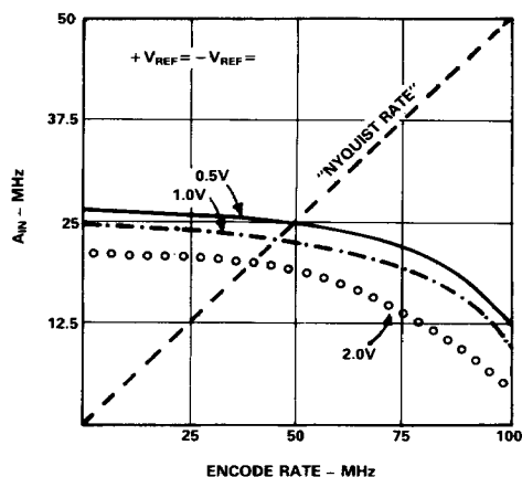
Analog Input vs. Encode Rate "No Missing Codes"
