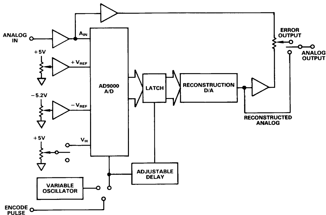
AD9000/PCB Block Diagram
