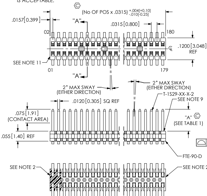
FIG 1 FTE-1XX-03-X-DV SHOWN
