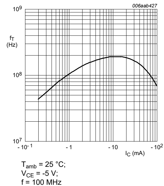
Fig. 15. PNP transistor: Transition frequency as a function of collector current; typical values
