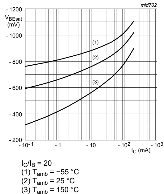
Fig. 13. PNP TR2: Base-emitter saturation voltage as a function of collector current; typical values
