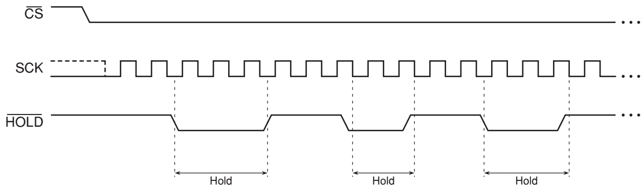
Figure 12-8. Hold Mode
