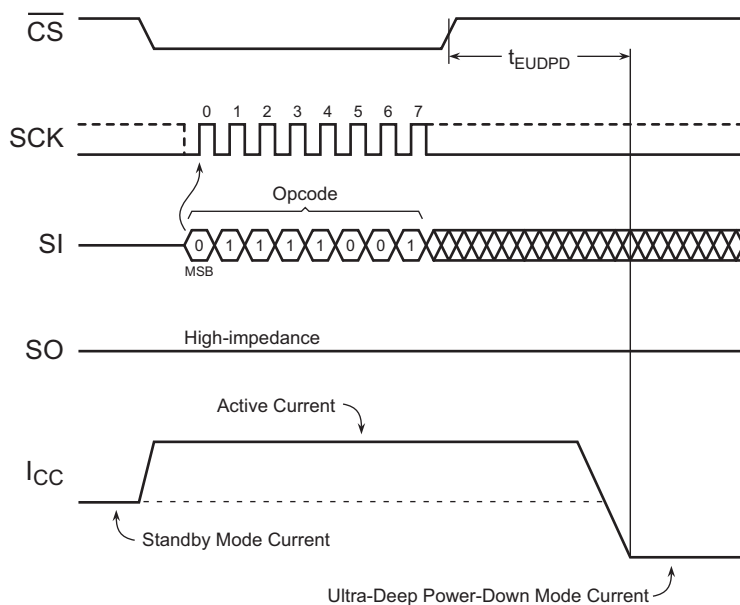
Figure 12-5. Ultra-Deep Power-Down
