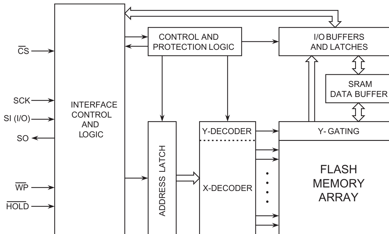
Figure 3-1. Block Diagram
