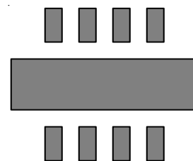
Figure 10 (c). Copper Area = 30mm 2 , \theta_{JA} = 54^{\circ}\text{C/W}
