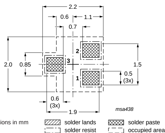
Fig 17. Reflow soldering footprint BAV70T (SOT416/SC-75)
