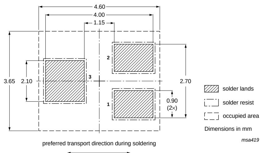
Fig 19. Wave soldering footprint BAV70W (SOT323/SC-70)
