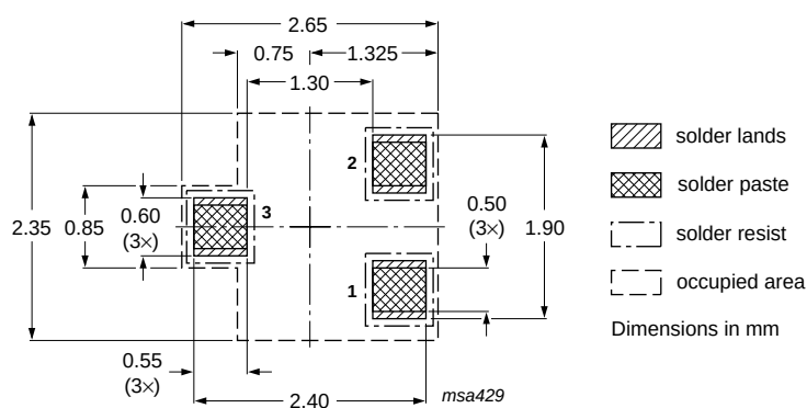
Fig 18. Reflow soldering footprint BAV70W (SOT323/SC-70)
