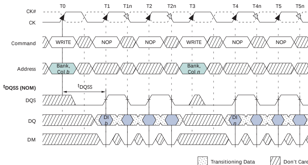
Figure 40: Nonconsecutive WRITE-to-WRITE
