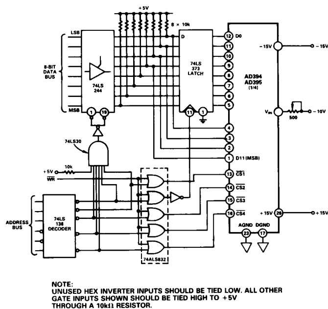
Figure 13. AD394, AD395 8-Bit Data Bus Interface
