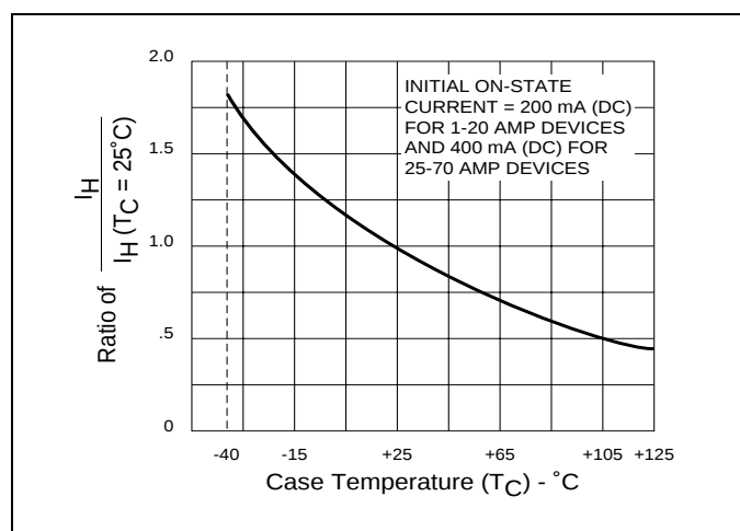
Figure 6.17 Normalized DC Holding Current vs Case Temperature
