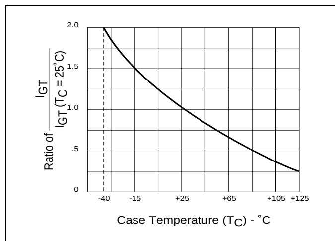
Figure 6.18 Normalized DC Gate-Trigger Current vs Case Temperature
