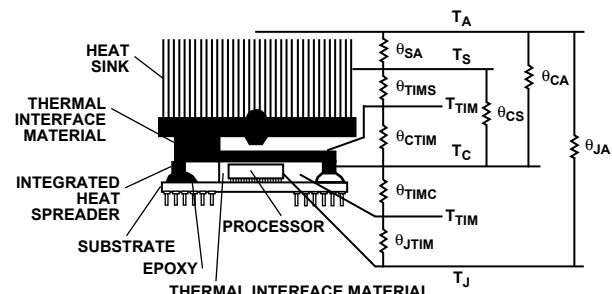
Figure 62. Thermal Model
