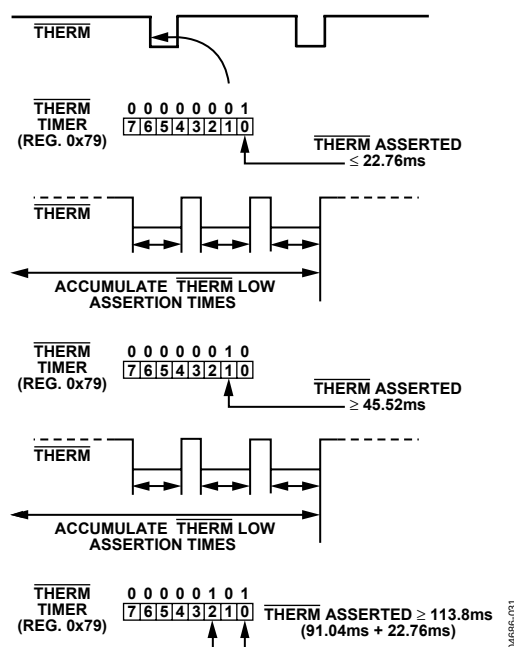
Figure 29. Understanding the \overline{\text{THERM}} Timer
