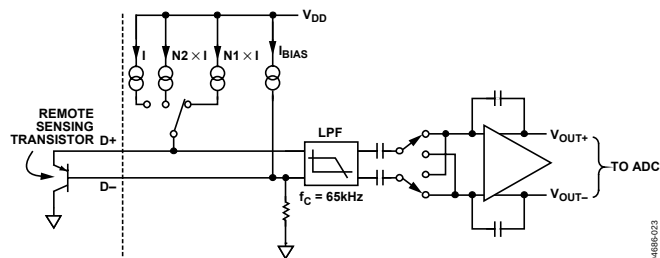
Figure 21. Signal Conditioning for Remote Diode Temperature Sensors
