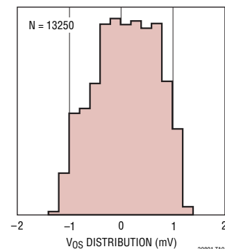
Offset Voltage Distribution
